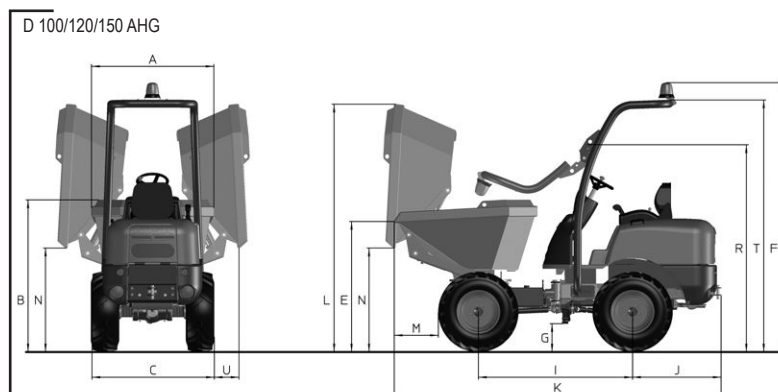
D 100/120/150 AHG
